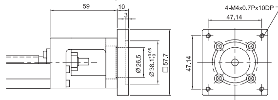
Motor Adaptor Flange F5
